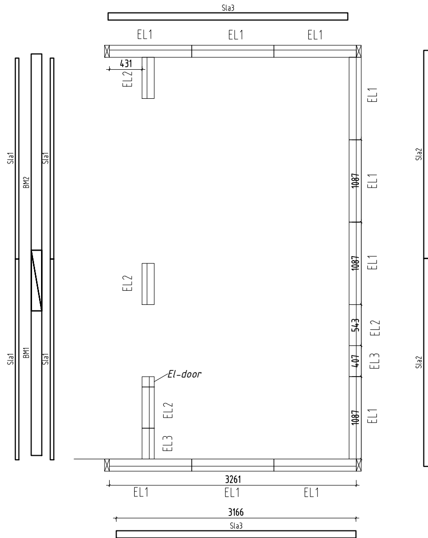
Wall panels position - Beams - Lath
